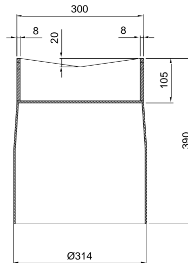
HUGOLINE Ø315
